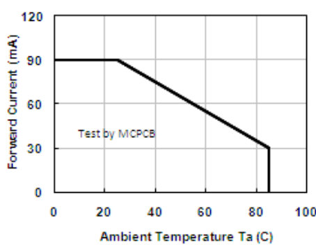
Fig.3 Forward Current Derating Curve
